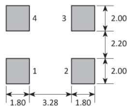
TOP VIEW Dimensions in mm
